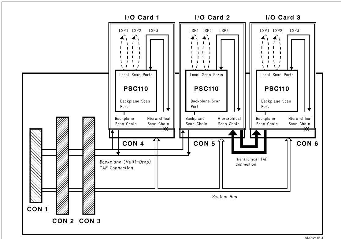
FIGURE 4. Backplane—Hierarchical Connection
