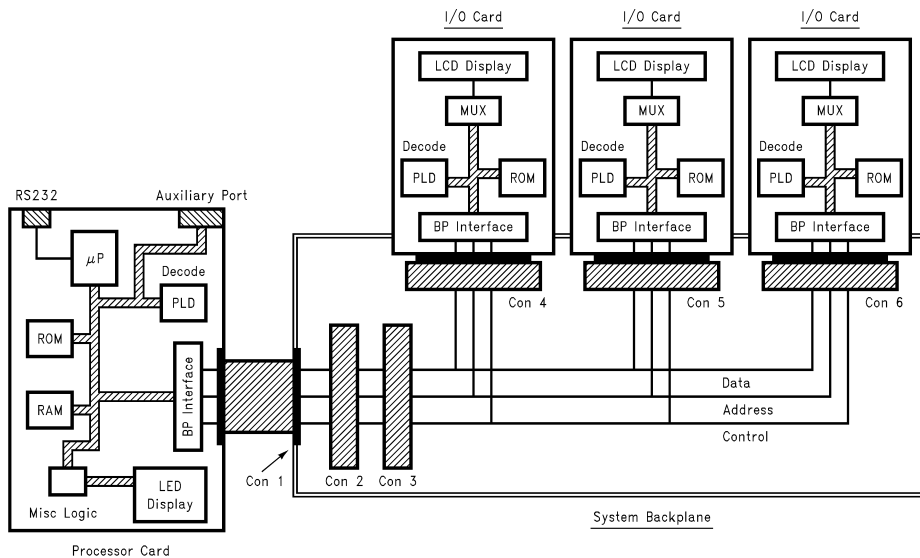
FIGURE 1. Demonstration System Layout
