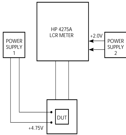
Figure 1. Test Setup
