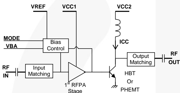
Figure 5. Block Diagram of a Typical WCDMA PA
