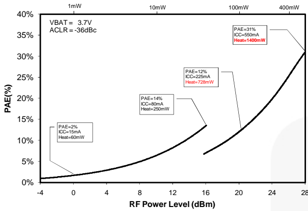
Figure 1. Power Added Efficiency (PAE) Variations in a Two-Mode WCDMA PA
