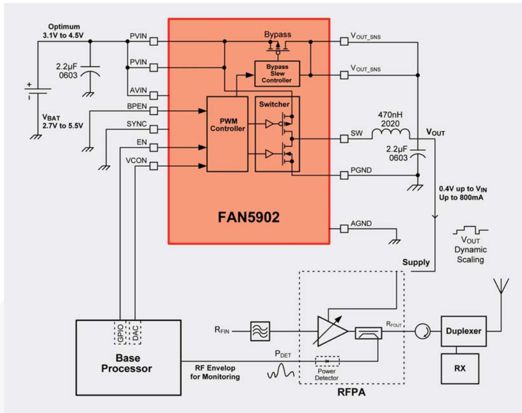
Figure 7. Typical Implementation of DVS for Improving PAE in WCDMA/UMTS RF Front-End
