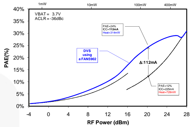
Figure 3. Power Added Efficiency (PAE) of Dual-Mode WCDMA PA with Integrated Duplexer (Black Curve) Compared to a Single-Mode PA Using Dynamic Voltage Supply (Blue Curve)
