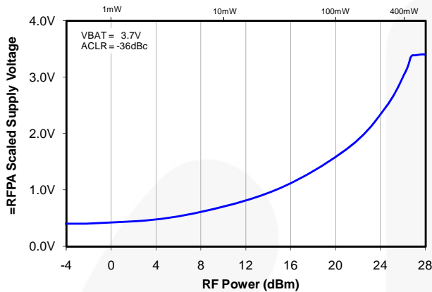
Figure 8. Typical Variations of the Supply Voltage Level Employed in a DVS Power Management Scheme for a WCDMA PA
