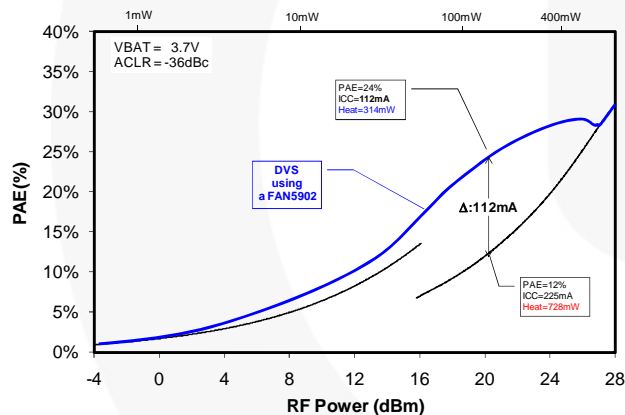
Figure 9. Improved PAE as a function of the Output Power Level for -36dBc ACLR
