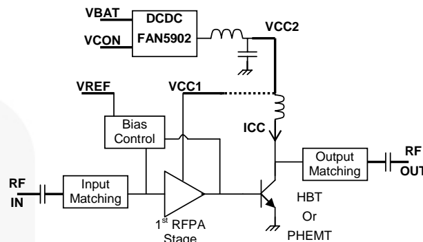
Figure 6. Block Diagram of a Typical WCDMA PA with a DC-to-DC Converter
