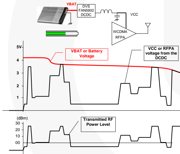
Figure 2. Dynamic Voltage Supply for 3G RF PA Using a DC-to-DC Converter
