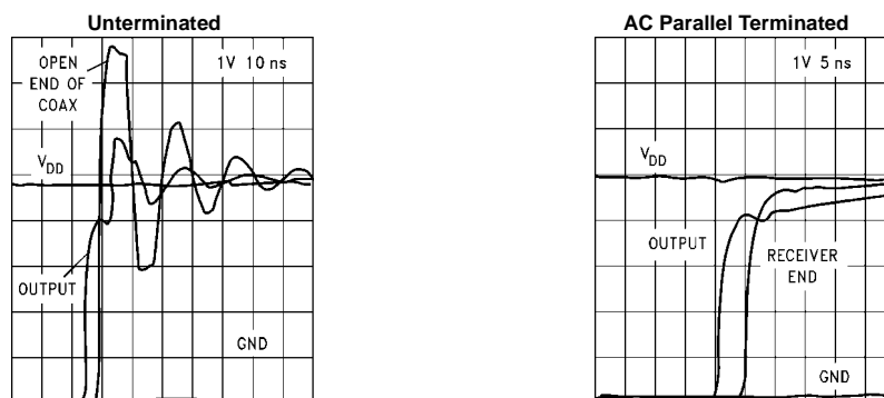
FIGURE 10. Terminating Transmission Lines
