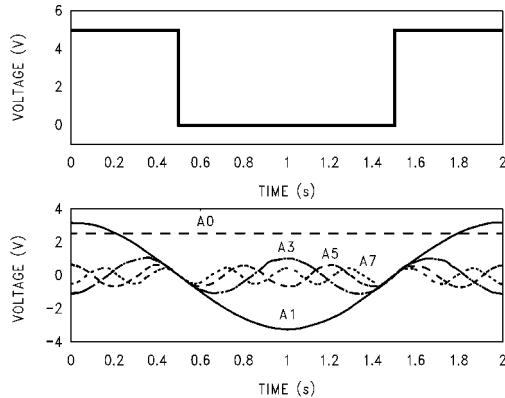
FIGURE 1. Square Wave with First Seven Harmonics
