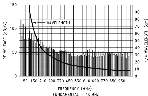
FIGURE 7. Example of DCM Method Spectral Content
