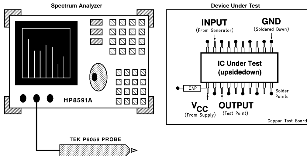
FIGURE 6. Direct Contact Measurement Method
