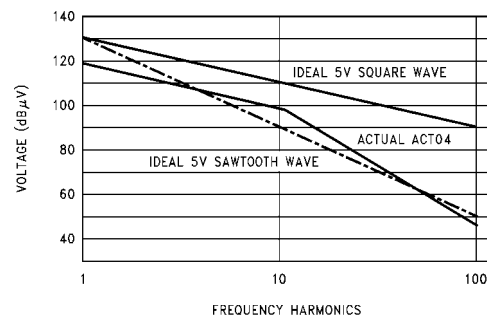
FIGURE 8. Ideal versus Actual Spectral Response
