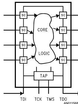
FIGURE 6. Exploiting the Boundary-Scan Test Logic to Also Test the Interior of an IC. IEEE 1149.1 Defines a Standard Instruction Called INTEST
