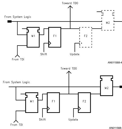
FIGURE 4. With IEEE 1149.1 I/O Pins May Capture the Data Arriving at a Pin and They May Be Used to Control Output Pins. Test Circuits Such as These May Also Test Internal System Logic. Circuits Such as These are Added to All System Pins
