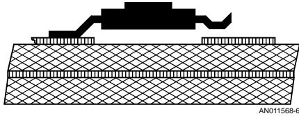
FIGURE 5. Lifted IC Leads, Not Accessible with Bed-of-Nails by the Embedded Probes of the Driving and Receiving IC, if they Implement Boundary-Scan
