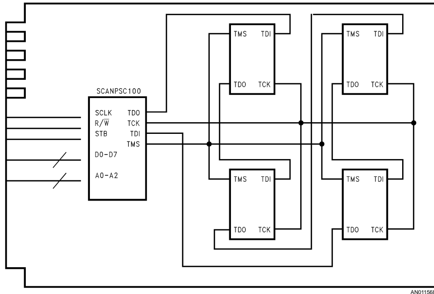
FIGURE 7. An Example of 1149.1 Applied to the Test Access of a PWB with No Spare Backplane Pins to Provide Test Access. A Typical Bus Master, SCANPSC100, Develops the Needed Test Port on the Module
