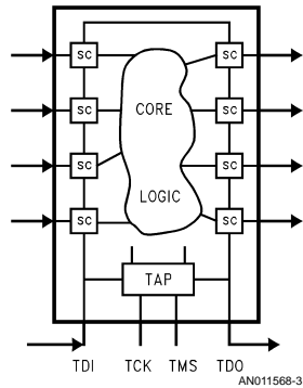
FIGURE 3. Bed-of-Nails Test Access Has Been Replaced by Adding Embedded Test Probes to Each IC Input and by Providing Test Drivers at Each Output. Driving Outputs and Sampling Inputs is Called EXTEXT
