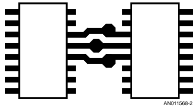
FIGURE 2. Despite Shrinking Component Sizes, Some Users Have Kept Large Feature-Sized Etch to Continue to Support Physical Access
