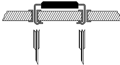
FIGURE 1. Traditional Bed-of-Nails PCB Test Access Method, Now Challenged by Shrinking Physical Contact Possibilities
