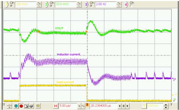
Figure 23. Load Transient, 0.1-3.0A Load, t_R=t_F=100ns , C_{OUT}=2x22\mu F
