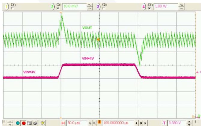
Figure 20. Line Transient, 50\Omega Load, t_R=t_F=10\mu s
