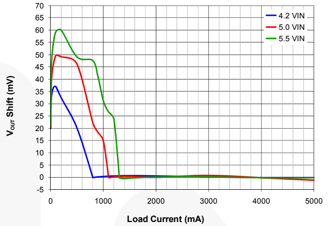
Figure 11. Regulation, 3.3V OUT
