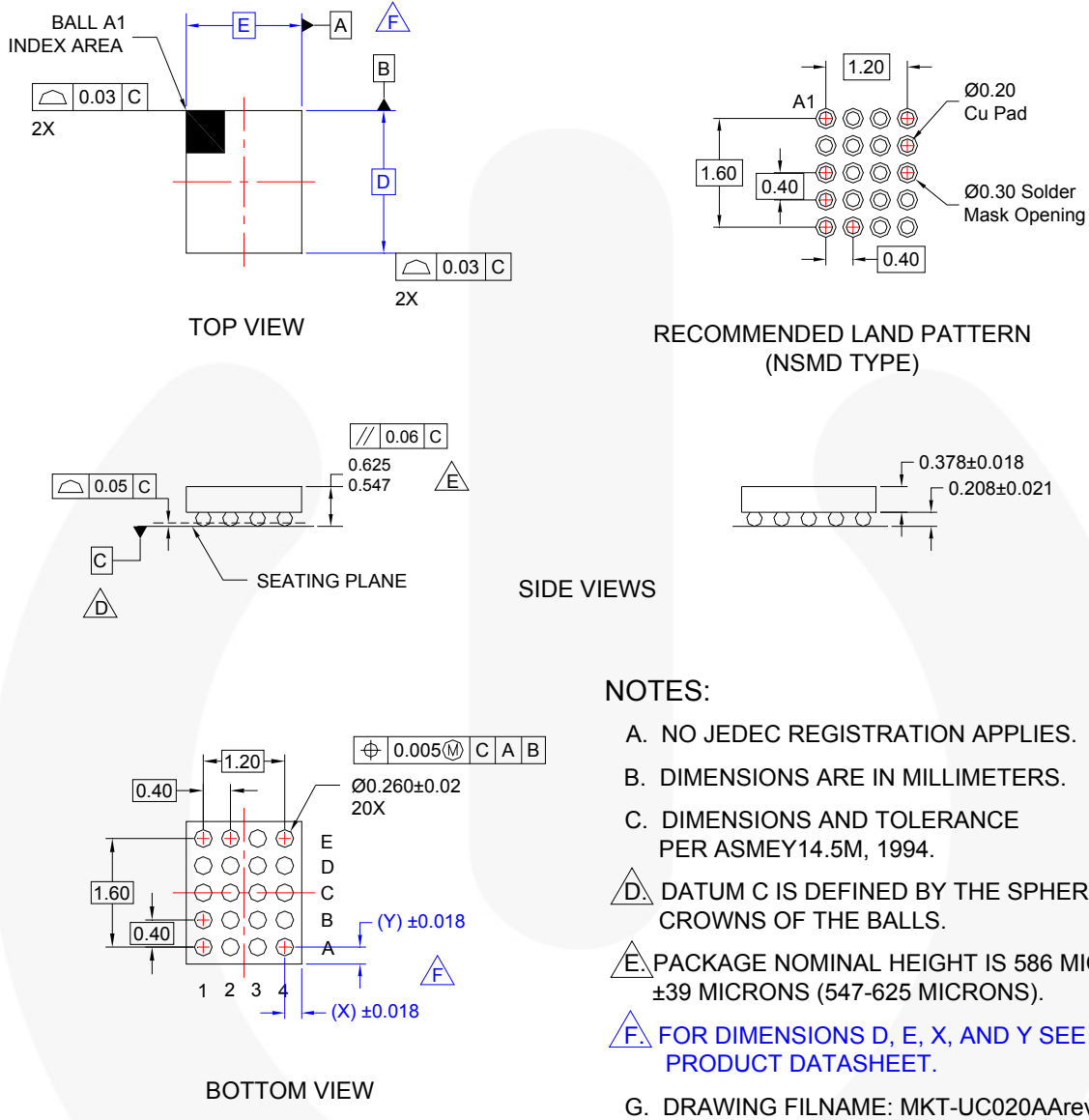
Figure 31 20-Ball WLCSP, 4x5 Array, 0.4mm Pitch, 250µm Ball
