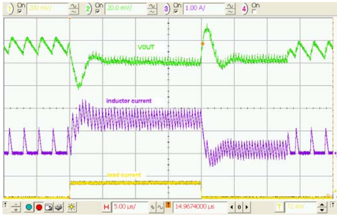
Figure 22. Load Transient, 0.1-1.5A Load, t_R=t_F=100ns
