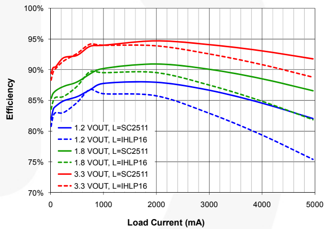
Figure 19. Inductor Efficiency Comparison, 5.0V_{IN}
