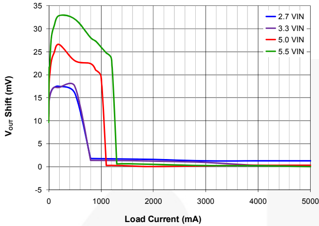
Figure 10. Regulation, 1.2V OUT
