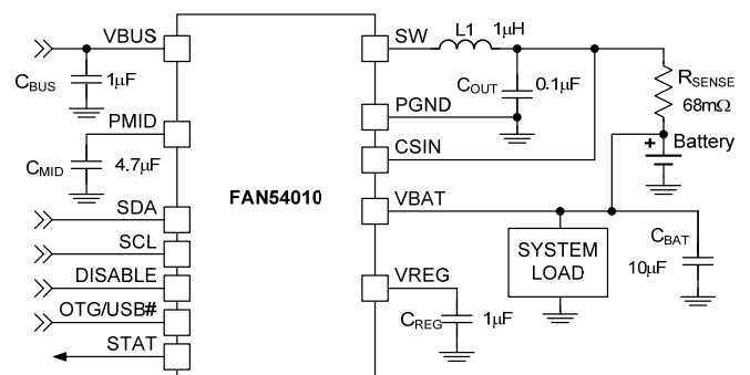
Figure 1. Typical Application
