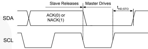
Figure 47. Stop Bit
