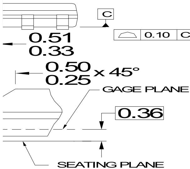
Figure 28. 8-Lead Small Outline Package (SOP)
