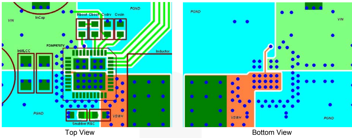
Figure 28. PCB Layout Example
