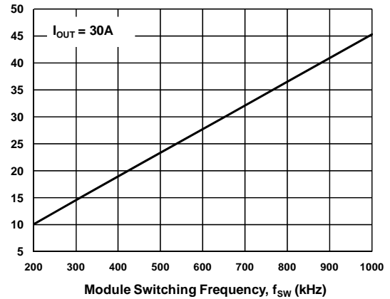
Figure 13. Driver Supply Current vs. Frequency
