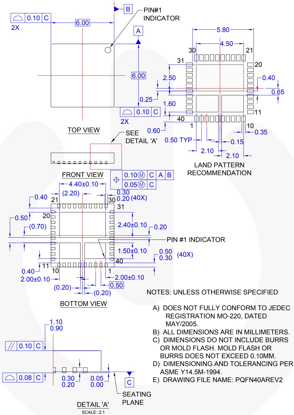
Figure 29. 40-Lead, Clipbond PQFN DrMOS, 6.0x6.0mm Package
