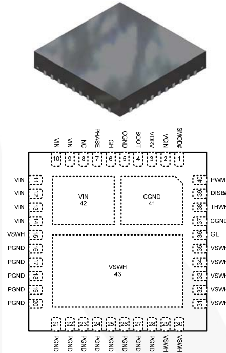
Figure 4. Top View
