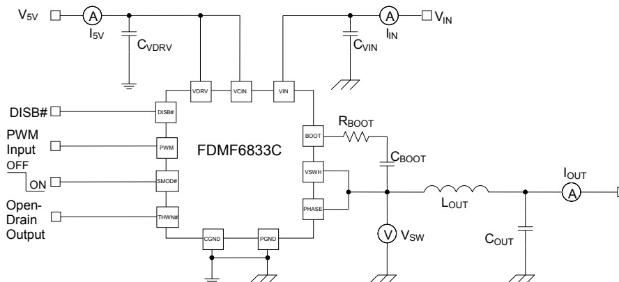
Figure 31. Block Diagram With V_{CIN} Filter
