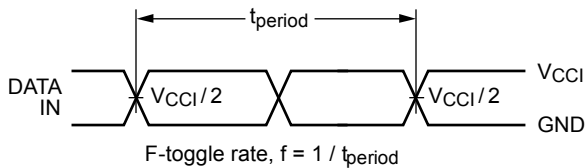
Figure 14. F-Toggle Rate
