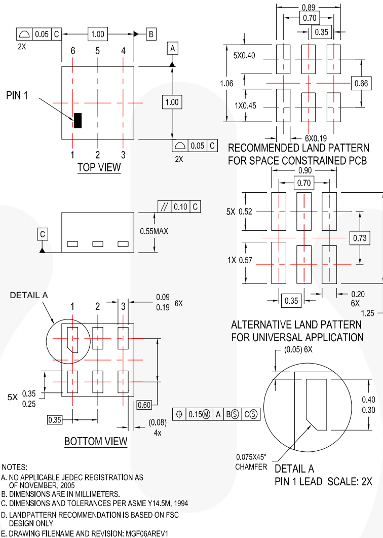
Figure 9. 6-Lead, MicroPak2, 1x1mm Body, .35mm Pitch
