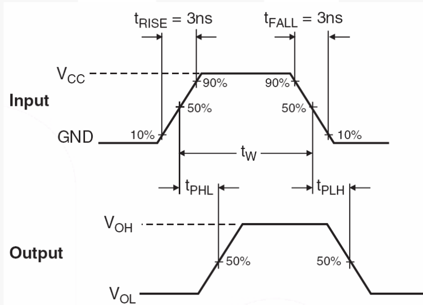
Figure 6. AC Waveforms
