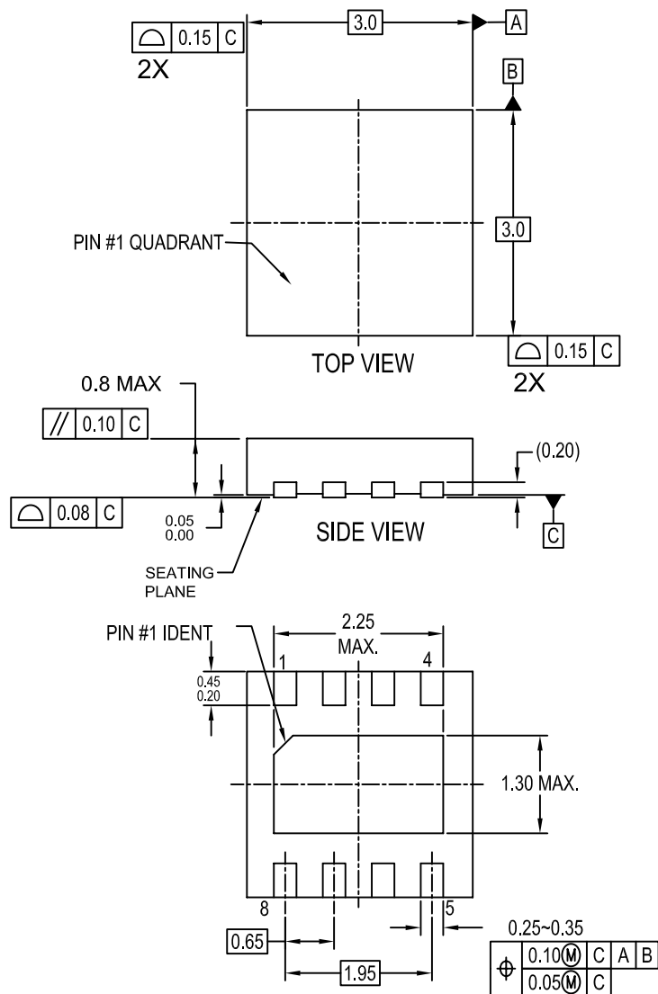
BOTTOM VIEW
