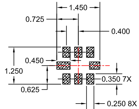
LAND PATTERN RECOMENDATION
