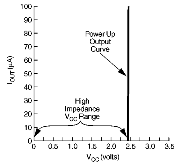
Port - I_{PU} Curve GTLP8T306
