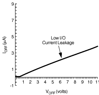
Port - I_{OFF} Curve GTLP8T306
