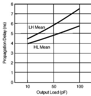
GTLP to TTL Propagation Delays (Single Output Switching) GTLP8T306
