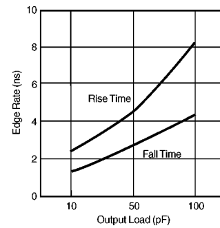
GTLP to TTL Output Edge Rates (Single Output Switching) GTLP8T306
