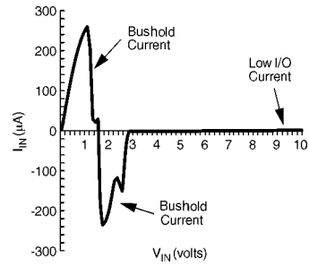
TTL Port - I_{IN} Curve GTLP8T306
