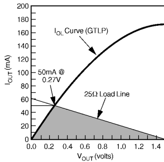
GTLP Port I_{OL} Curve with 25\Omega Load Line GTLP8T306
