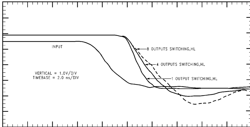
FIGURE 22. Multiple Output Switching, HL, 1, 4, 8 Outputs 74ABT244, V_{CC} = 5.0V , T_A = 25^\circ C
