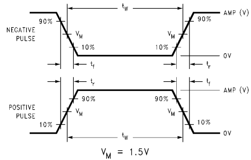
FIGURE 2. Test Input Signal Levels and Requirements
