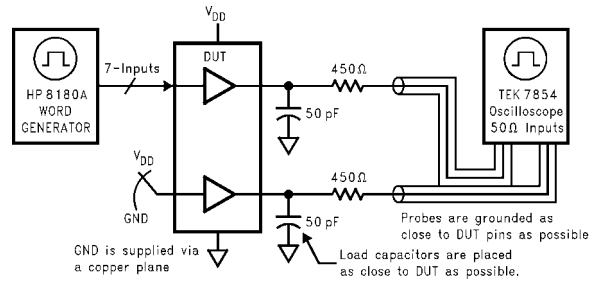
FIGURE 7. Simultaneous Switching Test Circuit
