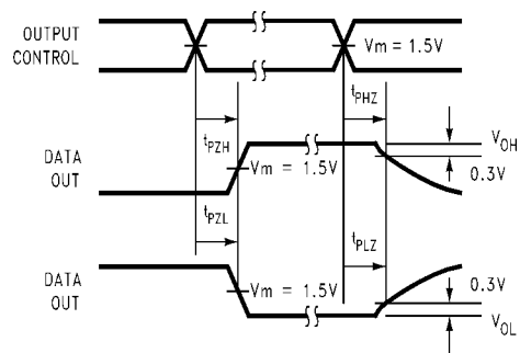
FIGURE 4. 3-STATE Output HIGH and LOW Enable and Disable Times
