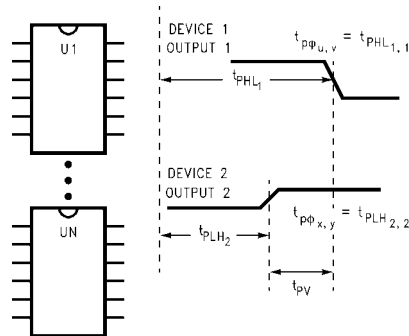
FIGURE 20. t_{PV}
