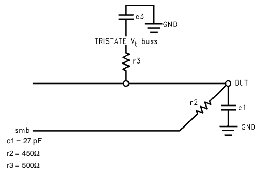
FIGURE 41. Output (3-STATE/Open Collector)
