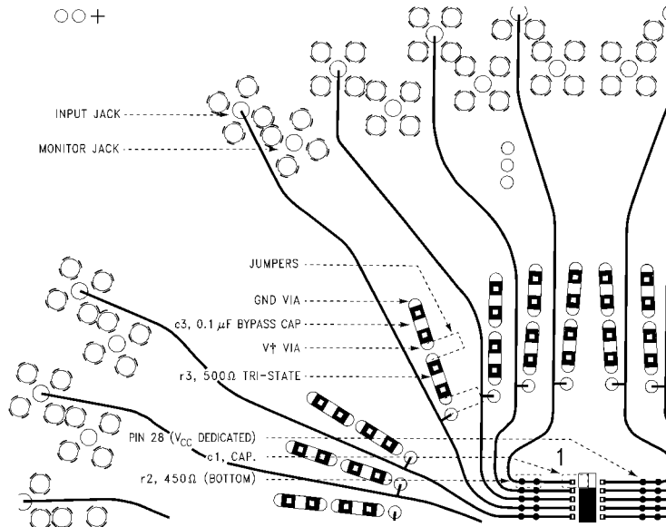
FIGURE 42. Component Placement on PC Board
