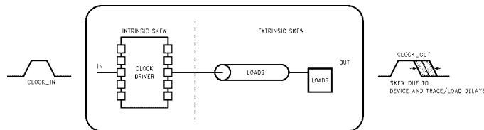
FIGURE 9. Sources of Clock Skew
