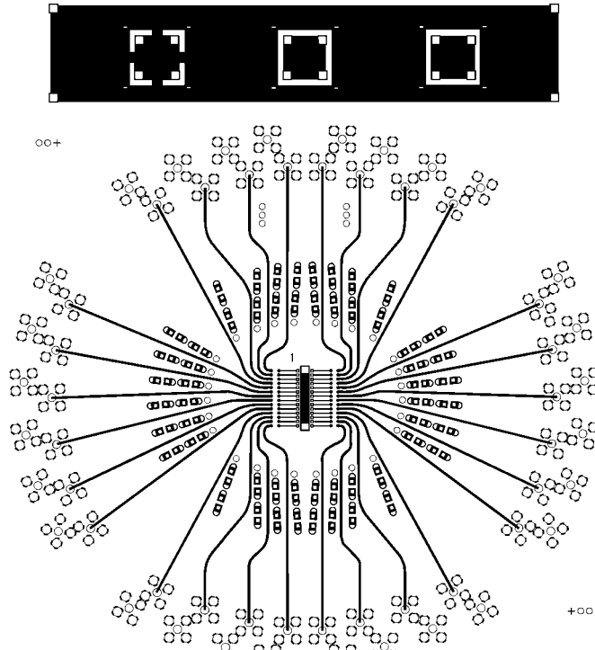
FIGURE 37. 28-Pin SOIC BOTTOM (Viewed from Top)
