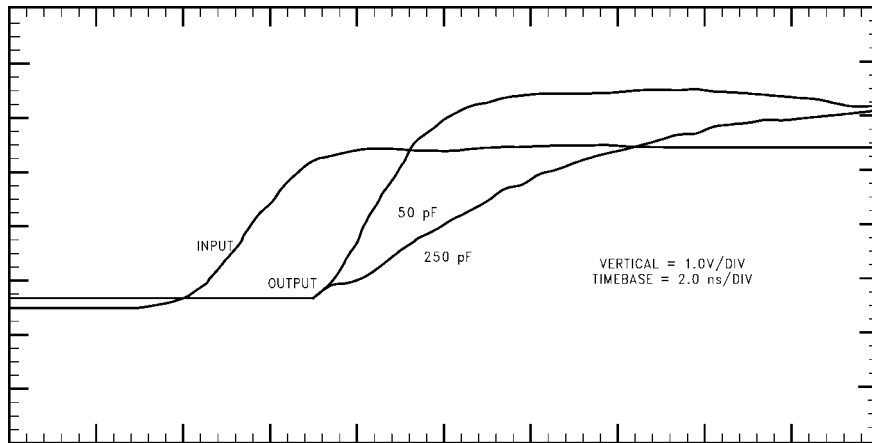
FIGURE 23. Single Output Switching, LH, 50 pF, 250 pF Capacitive Loading 74ABT244, V_{CC} = 5.0V , T_A = 25^\circ C
