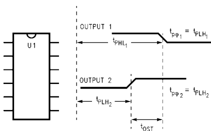
FIGURE 17. t_{OST}
