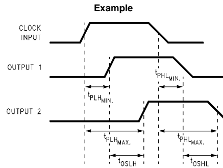
FIGURE 13. t_{OSLH} , t_{OSHL}
