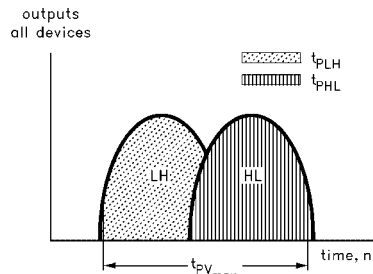
FIGURE 19. t_{PV}
