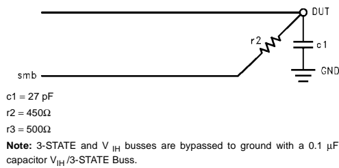
FIGURE 40. Output (2-State)
