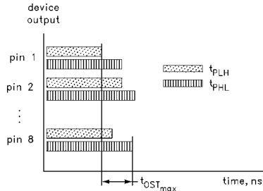
FIGURE 16. t_{OST}
