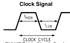
FIGURE 11. Clock Cycle
