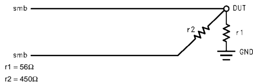
FIGURE 38. Input
