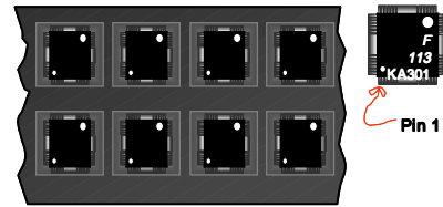
48-QFPH-1414 Unit Orientation
