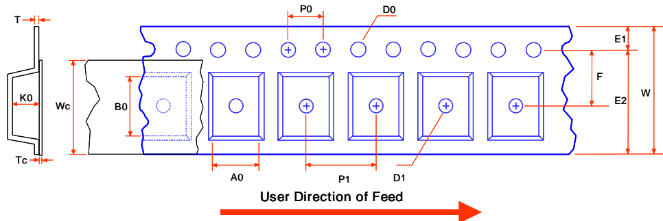
28-SSOPH-375-SG2 Embossed Carrier Tape Configuration: Figure 3.0
