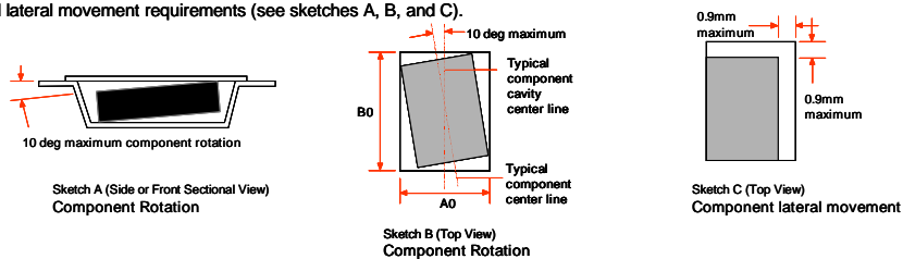
28-SSOPH-375-SG2 Reel Configuration: Figure 4.0
