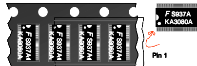
28-SSOPH-375-SG2 Unit Orientation
