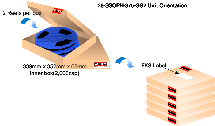
28-SSOPH-375-SG2 Unit Orientation
