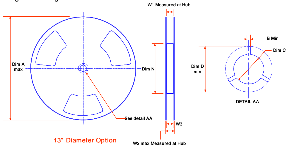
28-SSOPH-375-SG2 Reel Configuration: Figure 4.0
