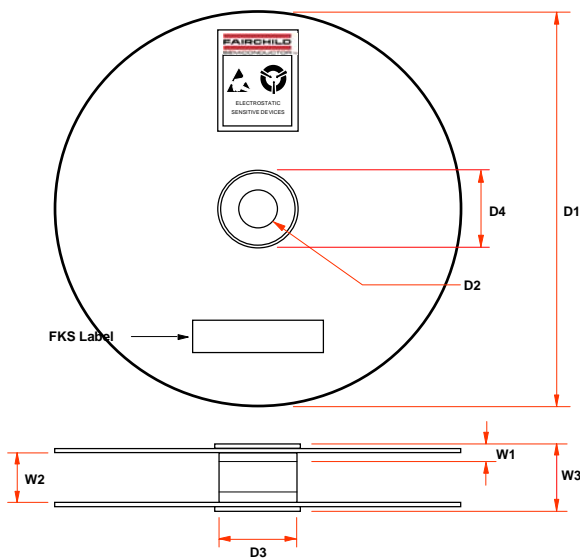
TO-92 Reel Configuration: Figure 8.0
