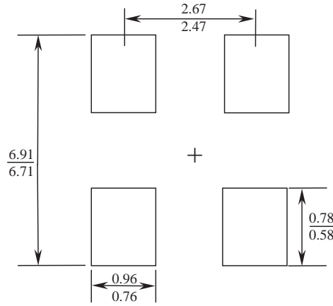
Minimum Recommended Land Pattern
