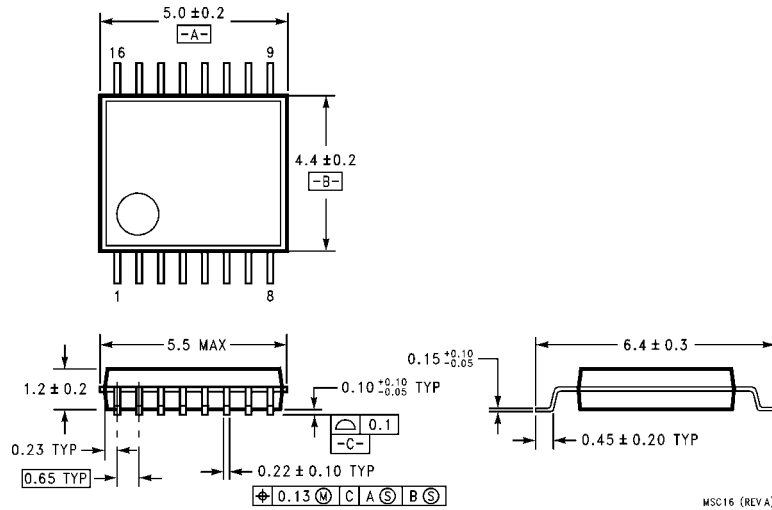
16-Lead Shrink Small Outline Package (SSOP), EIAJ TYPE I, 4.4mm Wide Package Number MSC16
