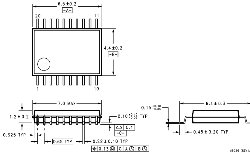
20-Lead Shrink Small Outline Package (SSOP), EIAJ TYPE I, 4.4mm Wide Package Number MSC20
