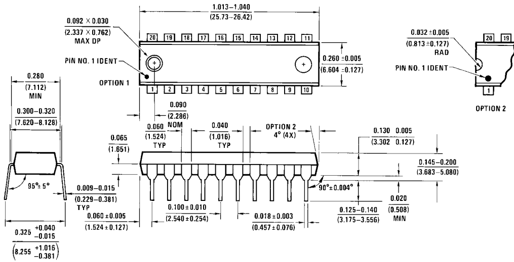
20-Lead Plastic Dual-In-Line Package (PDIP), JEDEC MS-001, 0.300" Wide Package Number N20
