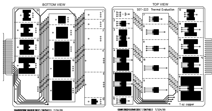
Figure 2. Both Sides of the 4.5"x5" SOT-223 Thermal Board. Complete scale drawings are shown in Section 5.
